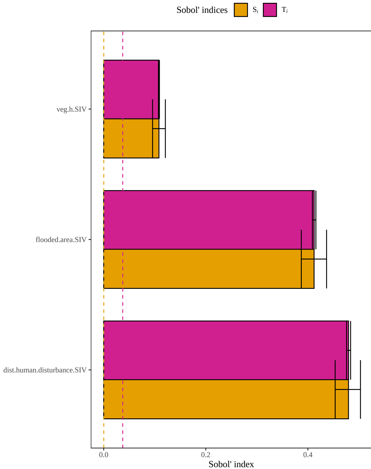
Figure 4. Results of a sensitivity analysis for the whiteibisWetland model based on an arithmetic mean structure. Dashed lines represent baseline numerical approximation error for S_i and T_i ( i.e. , dummy variables).
