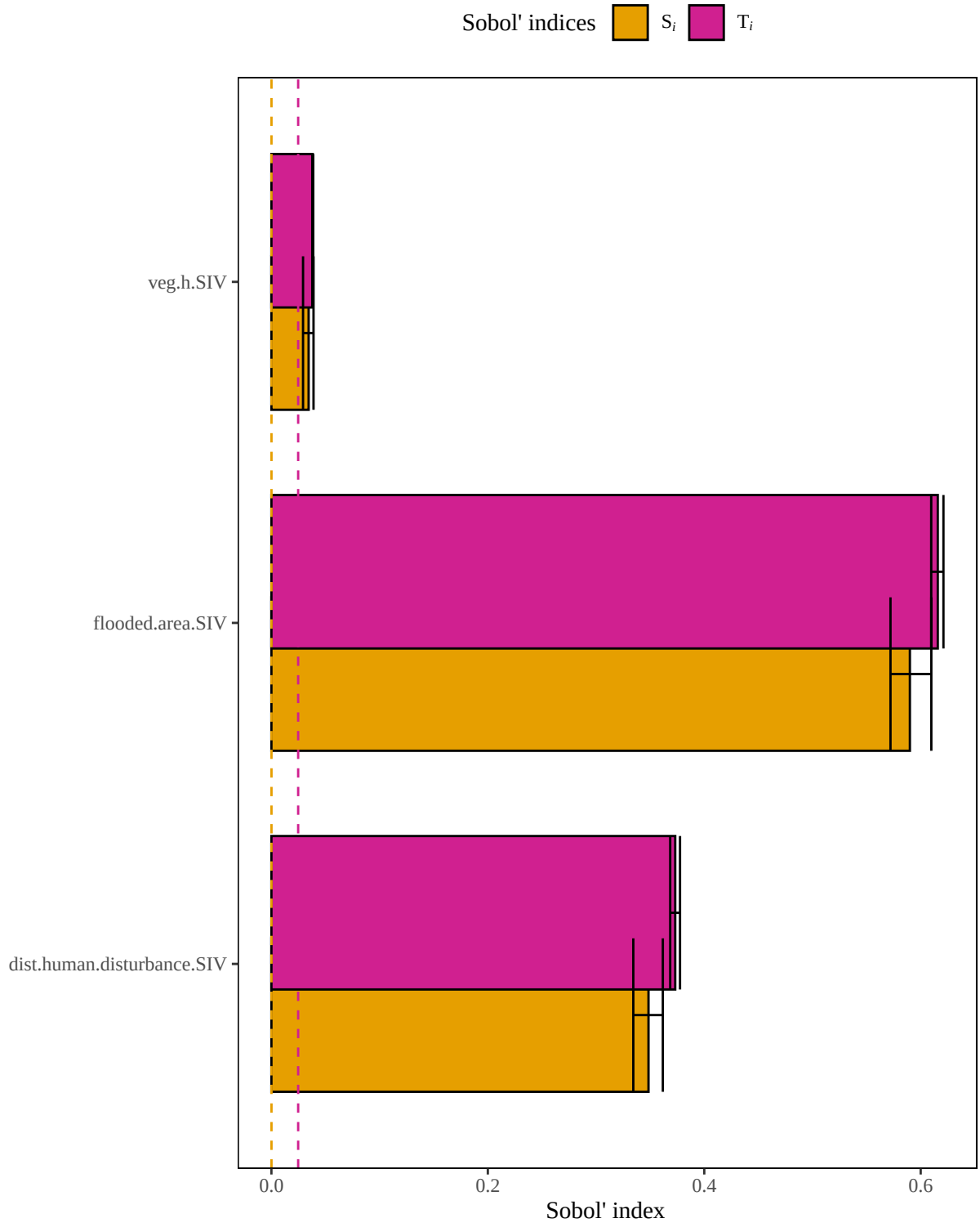
Figure 5. Results of a sensitivity analysis for the whiteibisWetland model based on a geometric mean structure. Dashed lines represent baseline numerical approximation error for S_i and T_i ( i.e. , dummy variables).
